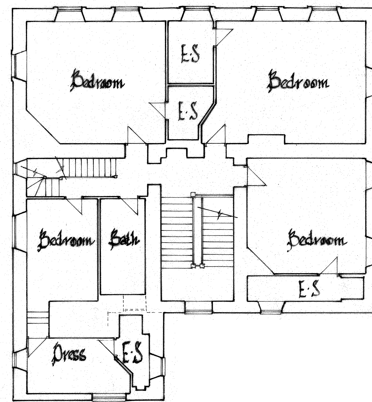
First Floor
